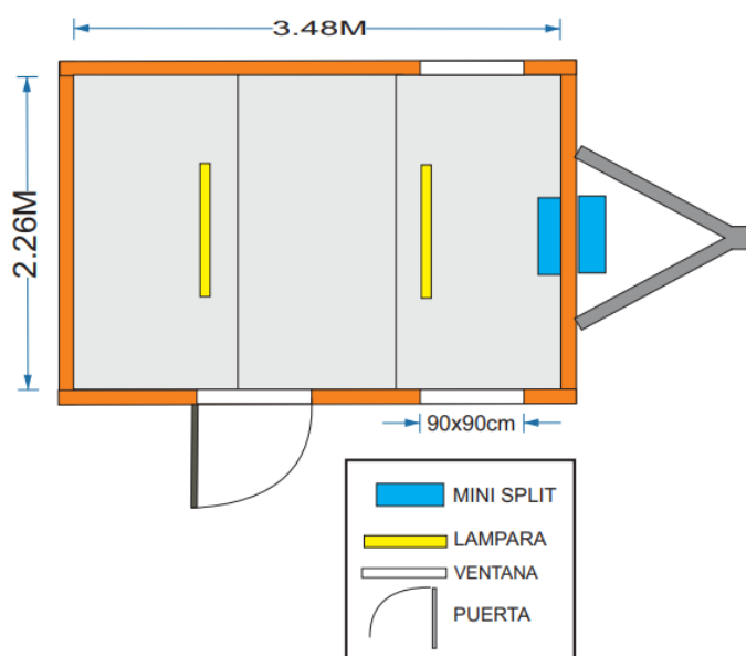
MODELO 08X16' 2.44 X 4.88 INTERIOR 2.26 X 3.48
